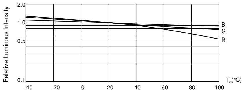
Fig. 5 Luminous Intensity at I_F = 20\text{mA} vs. Solder Point Temperature
