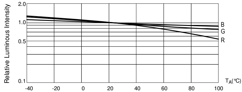
Fig. 5 Luminous Intensity at I_F=20mA vs. Ambient Temperature
