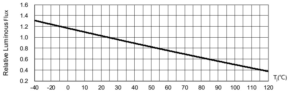
Fig. 5 Luminous Flux at I_F=30\text{mA} vs. Junction Temperature
