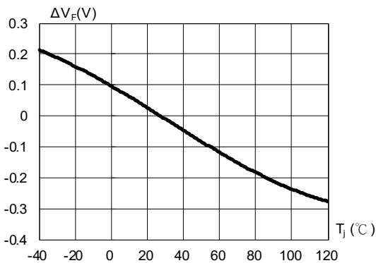
Fig. 3 Relative Forward Voltage vs. Junction Temperature \Delta V_F = V_F - V_F(25^\circ\text{C}) = f(T_j) ; I_F = 30\text{mA}
