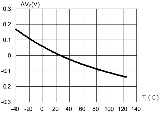
Fig. 3 Relative Forward Voltage vs. Junction Point Temperature \Delta V_F = V_F - V_F(25^\circ C) = f(T_J) ; I F = 50mA
