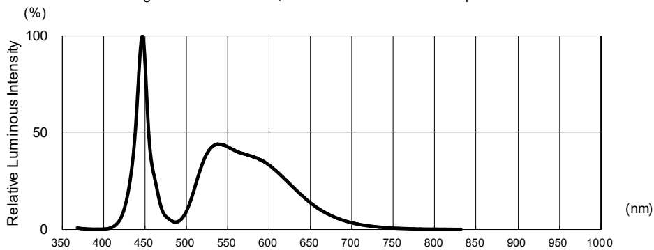
Fig.6. Relative Luminous Intensity vs. Wavelength
