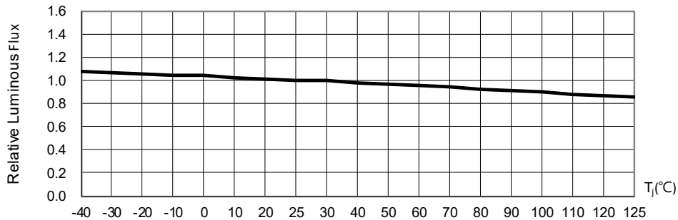
Fig. 5 Luminous Flux at I F =50mA vs. Junction Point Temperature
