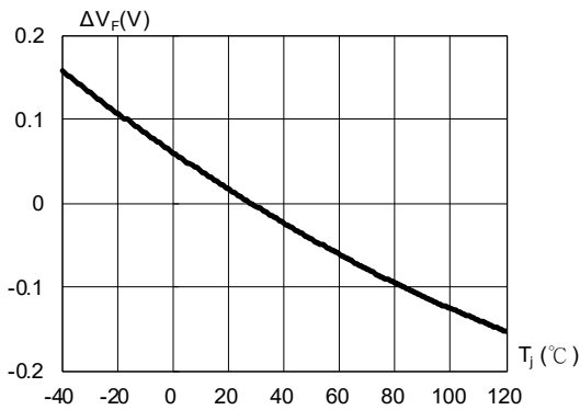
Fig. 3 Relative Forward Voltage vs. Junction Temperature \Delta V_F = V_F - V_F(25^\circ\text{C}) = f(T_s); I_F = 30\text{mA}
