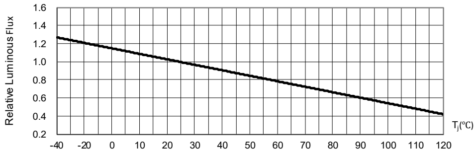
Fig. 5 Luminous Flux at I F =30mA vs. Junction Temperature
