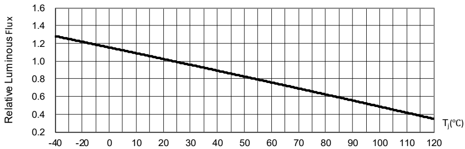
Fig. 5 Luminous Flux at I_F=30\text{mA} vs. Junction Temperature
