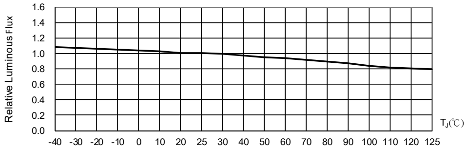
Fig. 5 Luminous Flux at I_F=50\text{mA} vs. Junction Point Temperature
