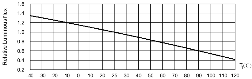
Fig. 5 Luminous Flux at I F =50mA vs. Junction Temperature
