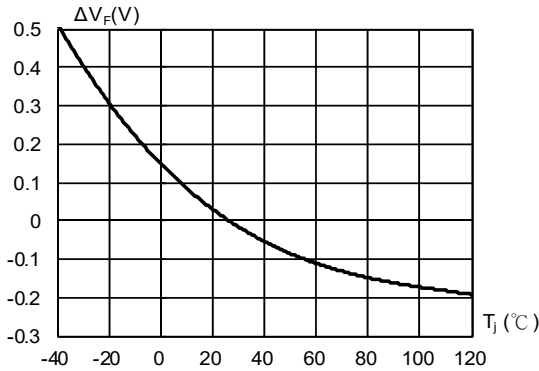
Fig. 3 Relative Forward Voltage vs. Junction Temperature \Delta V_F = V_F - V_F(25^\circ C) = f(T_s); I_F = 50mA
