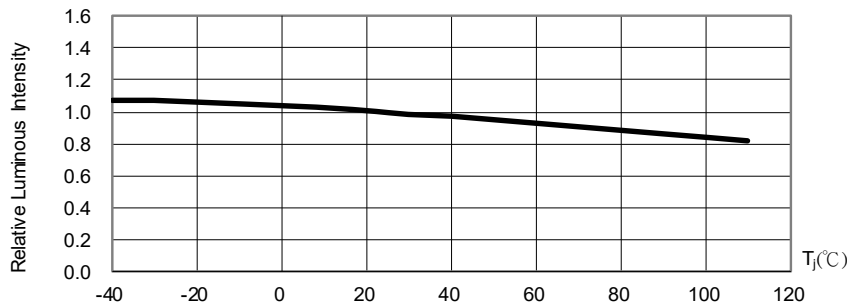
Fig. 5 Luminous Intensity at I_F=5\text{mA} vs. Junction Point Temperature
