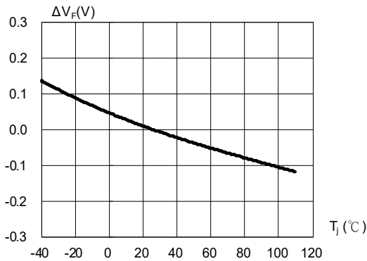
Fig. 3 Relative Forward Voltage vs. Junction Point Temperature \Delta V_F = V_F - V_F(25^\circ C) = f(T_J); I_F = 5mA
