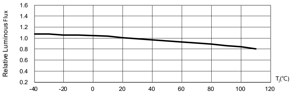
Fig. 5 Luminous Flux at I F =140mA vs. Junction Temperature
