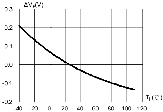
Fig. 3 Relative Forward Voltage vs. Junction Temperature \Delta V_F = V_F - V_F(25^\circ C) = f(T_J) ; I F = 140mA
