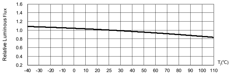
Fig. 5 Luminous Flux at I_F=50\text{mA} vs. Junction Temperature
