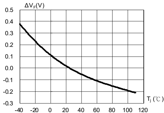
Fig. 3 Relative Forward Voltage vs. Junction Temperature \Delta V_F = V_F - V_F(25^\circ\text{C}) = f(T_J) ; I_F = 50\text{mA}
