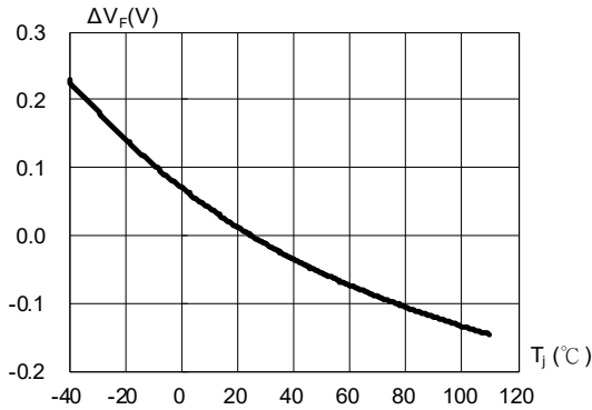
Fig. 3 Relative Forward Voltage vs. Junction Temperature \Delta V_F = V_F - V_F(25^\circ\text{C}) = f(T_s) ; I F = 140mA
