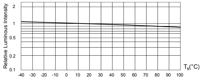
Fig. 5 Luminous Intensity at I_F=30mA vs. Solder Point Temperature
