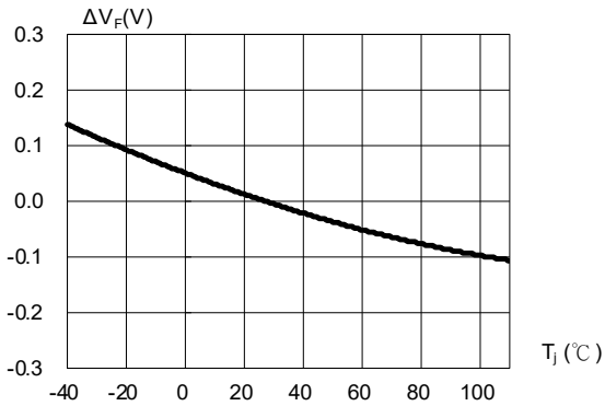
Fig. 3 Relative Forward Voltage vs. Junction Point Temperature \Delta V_F = V_F - V_F(25^\circ\text{C}) = f(T_J) ; I F = 20mA
