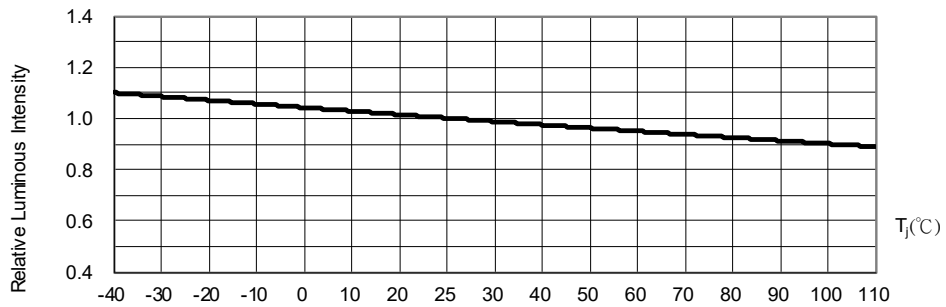
Fig. 5 Luminous Intensity at I F =20mA vs. Junction Point Temperature
