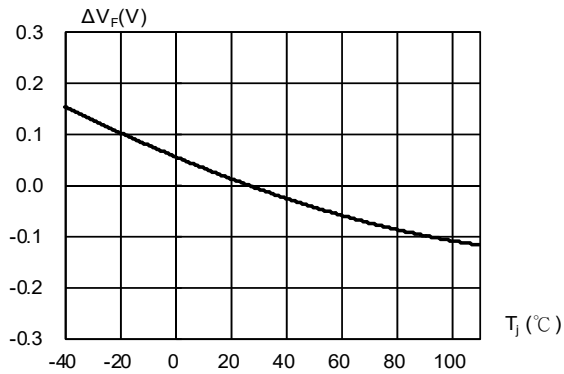
Fig. 3 Relative Forward Voltage vs. Junction Point Temperature \Delta V_F = V_F - V_F(25^\circ\text{C}) = f(T_J) ; I_F = 50\text{mA}
