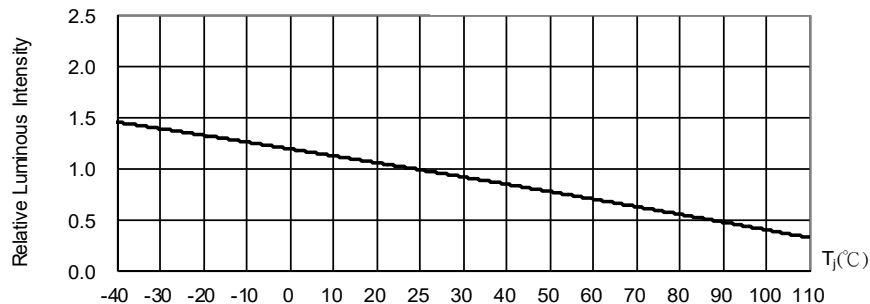
Fig. 5 Luminous Intensity at I_F=50\text{mA} vs. Junction Point Temperature
