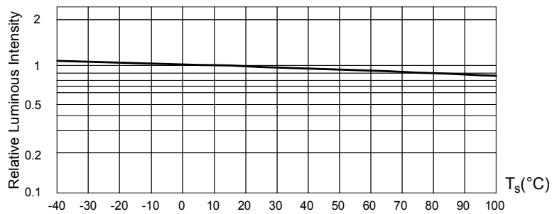
Fig. 5 Luminous Intensity at I_F=60mA vs. Solder Point Temperature
