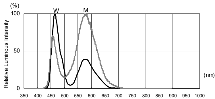
Fig. 6 Relative Luminous Intensity vs. Wavelength
