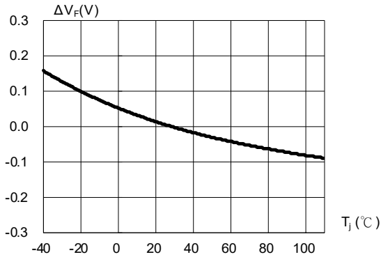
Fig. 3 Relative Forward Voltage vs. Junction Point Temperature \Delta V_F = V_F - V_F(25^\circ\text{C}) = f(T_J) ; I_F = 140\text{mA}
