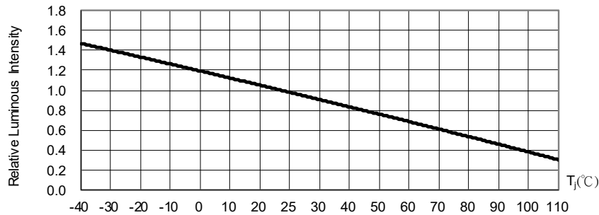
Fig. 5 Luminous Intensity at I_F=140\text{mA} vs. Junction Point Temperature
