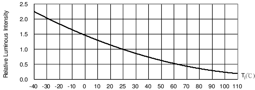
Fig. 5 Luminous Intensity at I F =140mA vs. Junction Point Temperature
