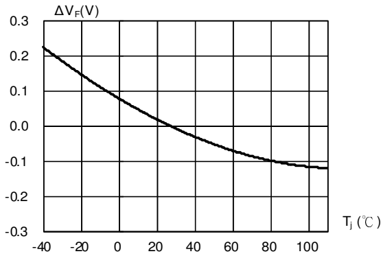
Fig. 3 Relative Forward Voltage vs. Junction Point Temperature \Delta V_F = V_F - V_F(25^\circ C) = f(T_J) ; I F = 140mA
