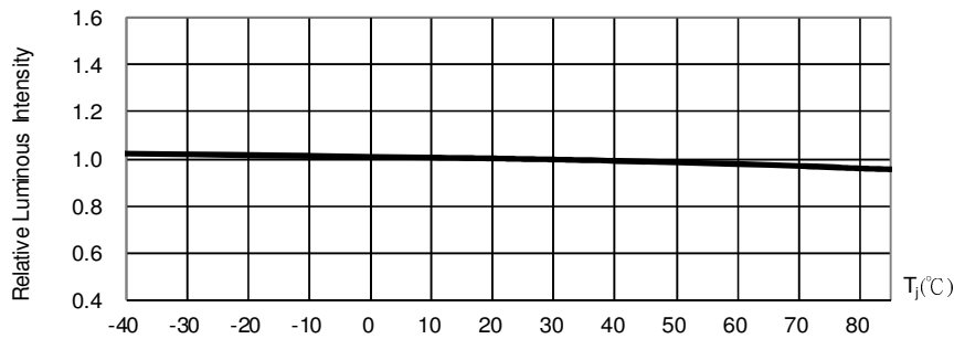
Fig. 5 Luminous Intensity at I F =20mA vs. Junction Point Temperature
