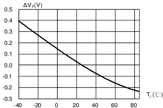
Fig. 3 Relative Forward Voltage vs. Junction Point Temperature \Delta V_F = V_F - V_F(25^\circ C) = f(T_J) ; I F = 20mA
