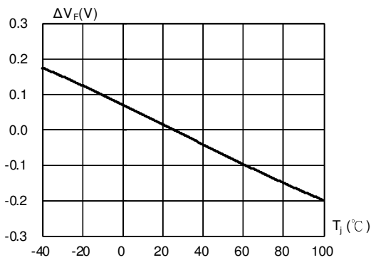
Fig. 3 Relative Forward Voltage vs. Junction Point Temperature \Delta V_F = V_F - V_F(25^\circ\text{C}) = f(T_J) ; I F = 20mA
