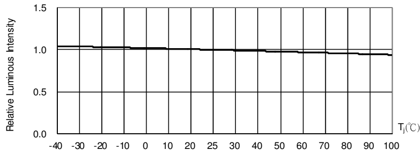
Fig. 5 Luminous Intensity at I F =20mA vs. Junction Point Temperature
