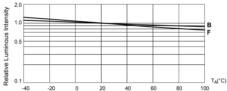
Fig. 5 Luminous Intensity at I_F=60mA vs. Ambient Temperature
