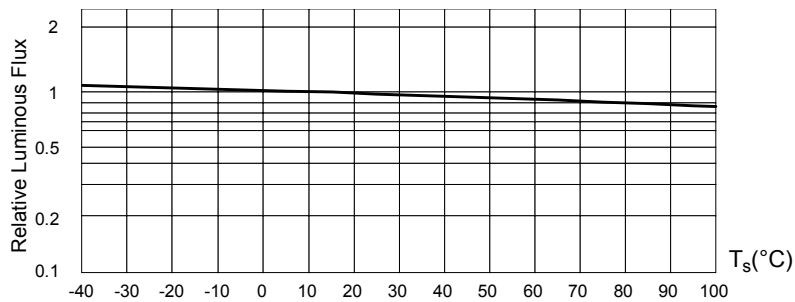
Fig. 5 Luminous Flux at I_F=60mA vs. Solder Point Temperature
