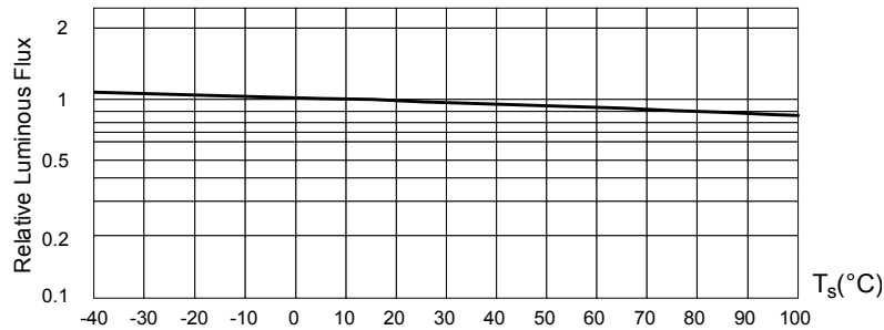
Fig. 5 Luminous Flux at I_F=150mA vs. Solder Point Temperature
