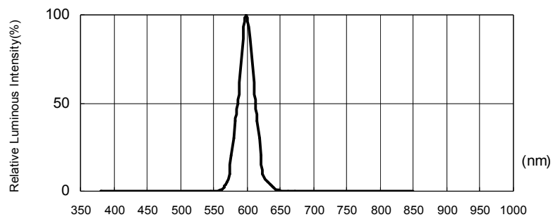
Fig 6. Relative Luminous Intensity vs. Wavelength
