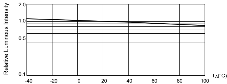
Fig. 5 Luminous Intensity at I_F = 20\text{mA} vs. Ambient Temperature
