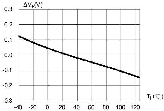
Fig. 3 Relative Forward Voltage vs. Junction Point Temperature \Delta V_F = V_F - V_F(25^\circ C) = f(T_j) ; I_F = 350mA
