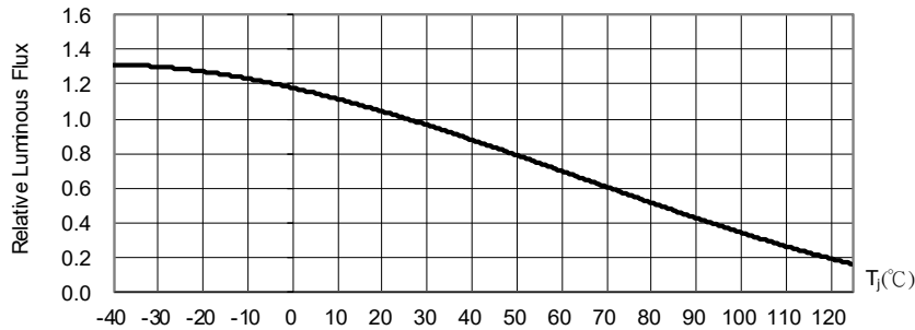
Fig. 5 Luminous Flux at I_F=350mA vs. Junction Point Temperature
