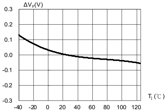
Fig. 3 Relative Forward Voltage vs. Junction Point Temperature \Delta V_F = V_F - V_F(25^\circ C) = f(T_j) ; I_F = 200\text{mA}
