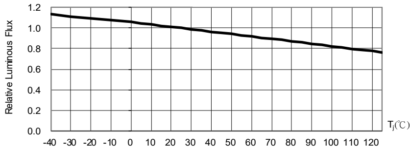
Fig. 5 Luminous Flux at I_F=200\text{mA} vs. Junction Point Temperature
