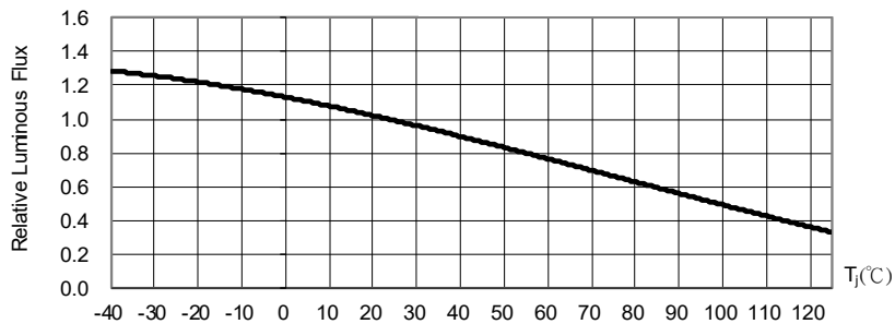
Fig. 5 Luminous Flux at I F =200mA vs. Junction Point Temperature
