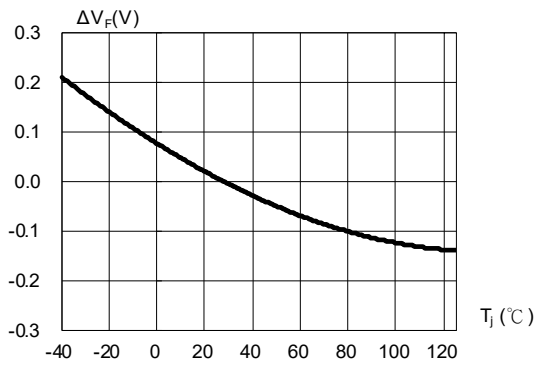
Fig. 3 Relative Forward Voltage vs. Junction Point Temperature \Delta V_F = V_F - V_F(25^\circ C) = f(T_J) ; I F = 200mA
