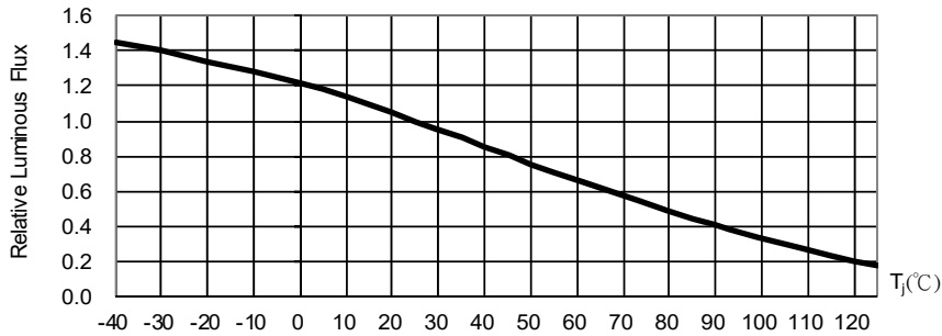
Fig. 5 Luminous Flux at I_F=200\text{mA} vs. Junction Point Temperature
