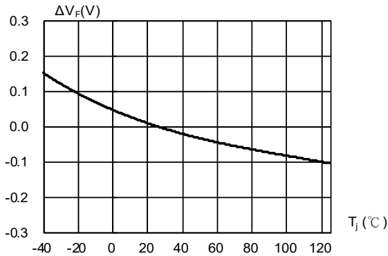
Fig. 3 Relative Forward Voltage vs. Junction Point Temperature \Delta V_F = V_F - V_F(25^\circ\text{C}) = f(T_j) ; I_F = 200\text{mA}
