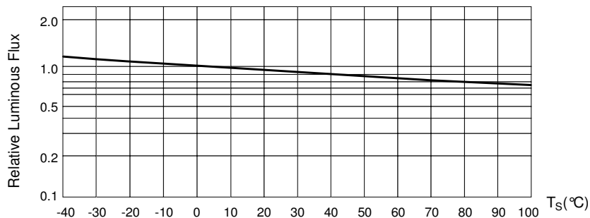
Fig. 5 Luminous Flux at I F =350mA vs. Solder Point Temperature
