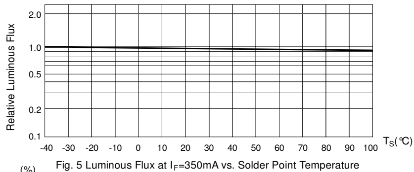
Fig.5 Luminous Flux at I_F=350mA vs. Solder Point Temperature
